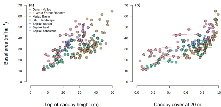
Figure 4. Relationship between field-measured basal area and (a) top-of-canopy height and (b) canopy cover at 20 m aboveground as measured through airborne laser scanning. Error bars correspond to standard deviations.
